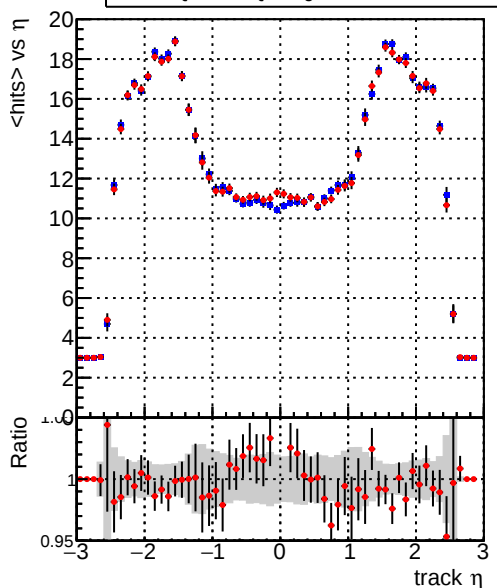
mean hits vs \eta Legend: DQM_CKF_QCDHighPt_base (blue line), DQM_CKF_QCDHighPt_retrainOldFiles125_v2_prelimWPM_epoch2 (red line)
