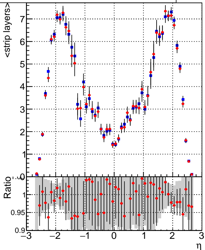
■ DQM_CKF_QCDHighPt_base ● DQM_CKF_QCDHighPt_retrainOldFiles125_v2_prelimWPM_epoch2
