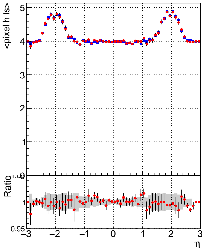
■ DQM_CKF_QCDHighPt_base ● DQM_CKF_QCDHighPt_retrainOldFiles125_v2_prelimWPM_epoch2
