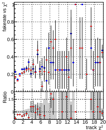
Fake rate vs. \chi^2 vs. \chi^2
