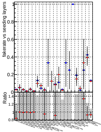
Fake rate vs. ◆ DQM_CKF_QCDHighPt_base ◆ DQM_CKF_QCDHighPt_retrainOldFiles125_v2_prelimWPM_epoch2
