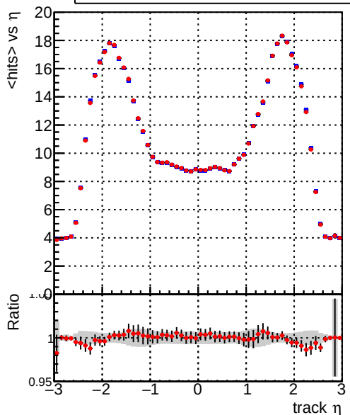
mean hits — DQM_CKF_QCDHighPt_base — DQM_CKF_QCDHighPt_retrainOldFiles125_v2_prelimWPM_epoch2
