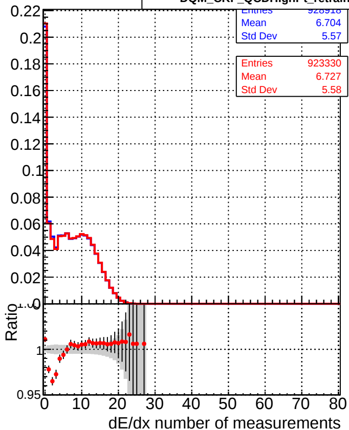
DQM_CKF_QCDHighPt_base DQM_CKF_QCDHighPt_retrainOldFiles125_v2_prelimWPM_epoch2
