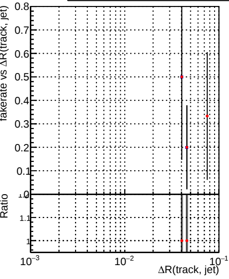
Legend: DQM_CKF_QCDHighPt_base (blue), DQM_CKF_QCDHighPt_retrainOldFiles125_v2_prelimWPM_epoch2 (red)
