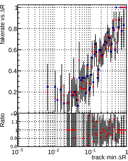
Legend: DQM_CKF_QCDHighPt_base (blue), DQM_CKF_QCDHighPt_retrainOldFiles125_v2_prelimWPM_epoch2 (red)
