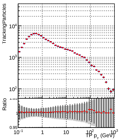
Legend: DQM_CKF_QCDHighPt_base (grey bars), DQM_CKF_QCDHighPt_retrainOldFiles125_v2_prelimWPM_epoch2 (red dots)
