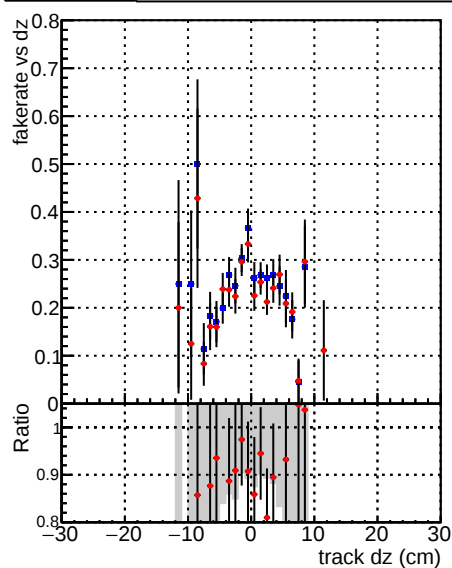
—●— DQM_CKF_QCDHighPt_base —●— DQM_CKF_QCDHighPt_retrainOldFiles125_v2_prelimWPM_epoch2
