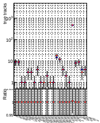
N of reco track vs. \chi^2 — DQM_CKF_QCDHighPt_base — DQM_CKF_QCDHighPt_retrainOldFiles125_v2_prelimWPM_epoch2
