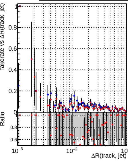
Legend: —•— DQM_CKF_QCDHighPt_base —•— DQM_CKF_QCDHighPt_retrainOldFiles125_v2_prelimWPM_epoch2
