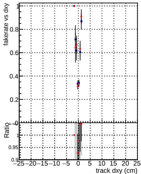
—●— DQM CKF QCDHighPt_base —●— DQM CKF QCDHighPt_retrainOldFiles125_v2_prelimWPM_epoch2
