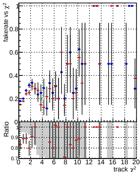
Fake rate vs. \chi^2 —◆— DQM_CKF_QCDHighPt_base —●— DQM_CKF_QCDHighPt_retrainOldFiles125_v2_prelimWPM_epoch2
