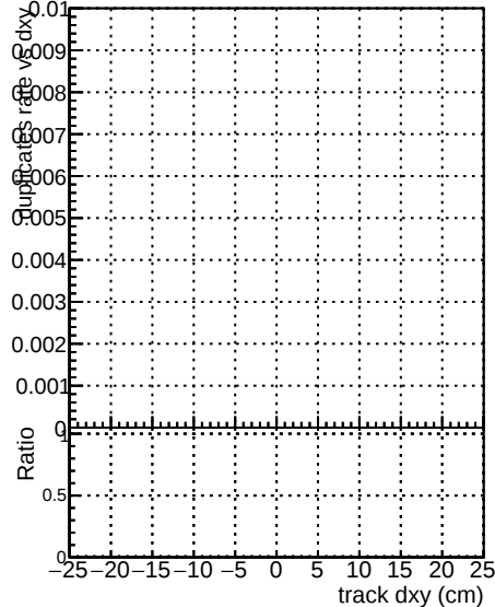
—■— DQM_CKF_QCDHighPt_base —●— DQM_CKF_QCDHighPt_retrainOldFiles125_v2_prelimWPM_epoch2
