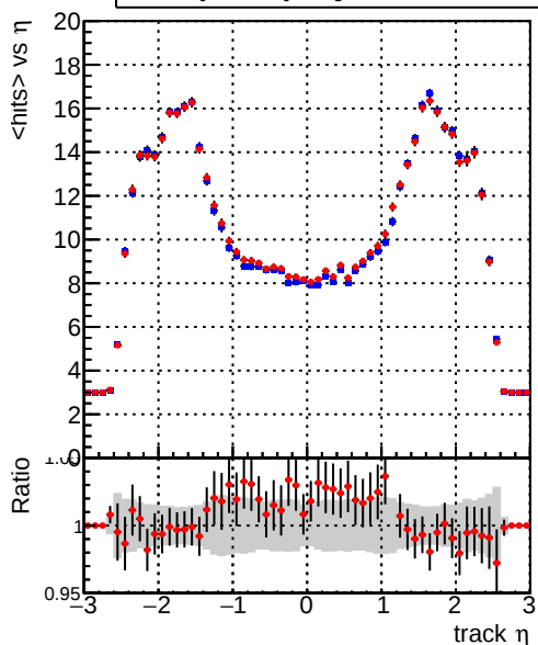
— DQM_CKF_QCDHighPt_base — DQM_CKF_QCDHighPt_retrainOldFiles125_v2_prelimWPM_epoch2
