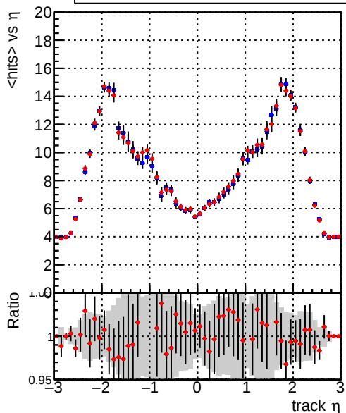
mean hits — DQM_CKF_QCDHighPt_base — DQM_CKF_QCDHighPt_retrainOldFiles125_v2_prelimWPM_epoch2
