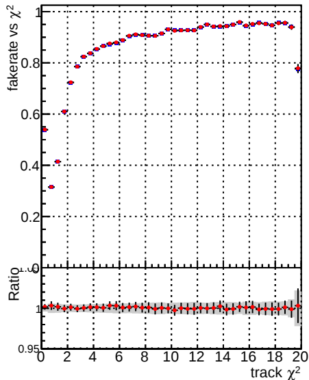
Fake rate vs. —•— DQM_CKF_QCDHighPt_base —•— DQM_CKF_QCDHighPt_retrainOldFiles125_v2_prelimWPM_epoch2
