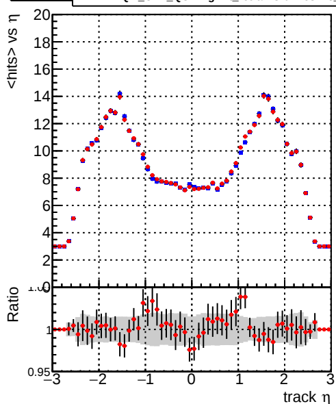
— DQM_CKF_QCDHighPt_base — DQM_CKF_QCDHighPt_retrainOldFiles125_v2_prelimWPM_epoch2
