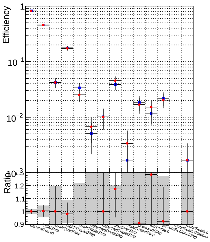
DQM_CKF_QCDHighPt_base DQM_CKF_QCDHighPt_retrainOldFiles125_v2_prelimWPM_epoch2
