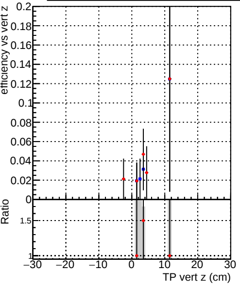
Efficiency vs TP vert z (cm) Legend: DQM_CKF_QCDHighPt_base (blue dots) DQM_CKF_QCDHighPt_retrainOldFiles125_v2_prelimWPM_epoch2 (red dots)
