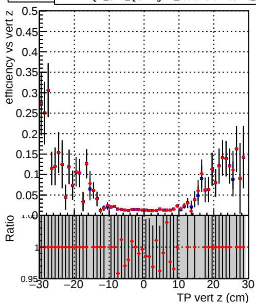
Efficiency vs TP vert z — DQM_CKF_QCDHighPt_base — DQM_CKF_QCDHighPt_retrainOldFiles125_v2_prelimWPM_epoch2
