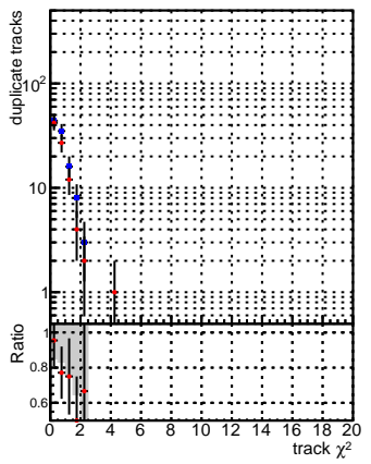
N of reco track vs. \chi^2 DQM_CKF_QCDHighPt_base DQM_CKF_QCDHighPt_retrainOldFiles125_v2_prelimWPM_epoch2 overSet
