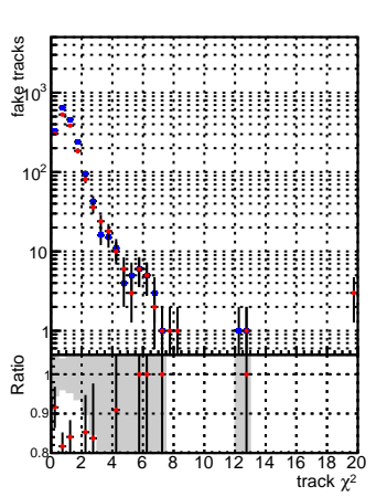
N of reco track vs. \chi^2 DQM_CKF_QCDHighPt_base DQM_CKF_QCDHighPt_retrainOldFiles125_v2_prelimWPM_epoch2 overSet
