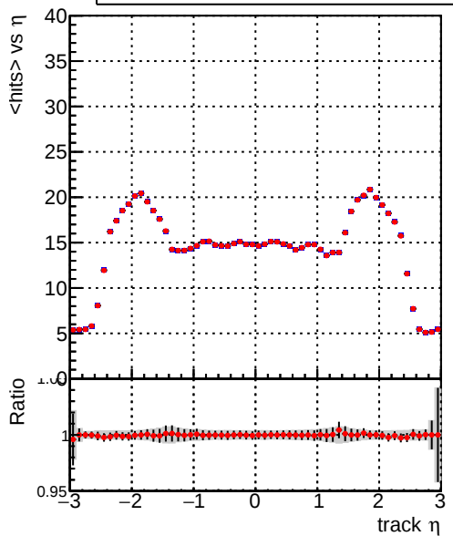
mean hits vs \eta — DQM_CKF_QCDHighPt_base — DQM_CKF_QCDHighPt_retrainOldFiles125_v2_prelimWPM_epoch2
