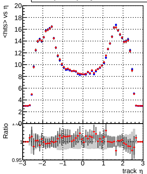
— DQM_CKF_QCDHighPt_base — DQM_CKF_QCDHighPt_retrainOldFiles125_v2_prelimWPM_epoch2
