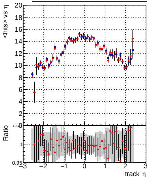
mean hits — DQM_CKF_QCDHighPt_base — DQM_CKF_QCDHighPt_retrainOldFiles125_v2_prelimWPM_epoch2
