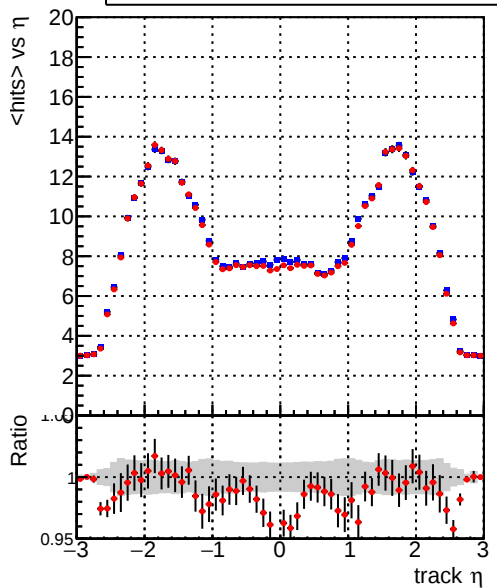
mean hit — DQM_CKF_QCDHighPt_base — DQM_CKF_QCDHighPt_retrainOldFiles125_v2_prelimWPM_epoch2
