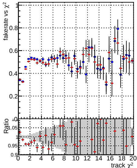
Fake rate vs. Legend: —•— DQM CKF_QCDHighPt_base —+— DQM CKF_QCDHighPt_retrainOldFiles125_v2_prelimWPM_epoch2
