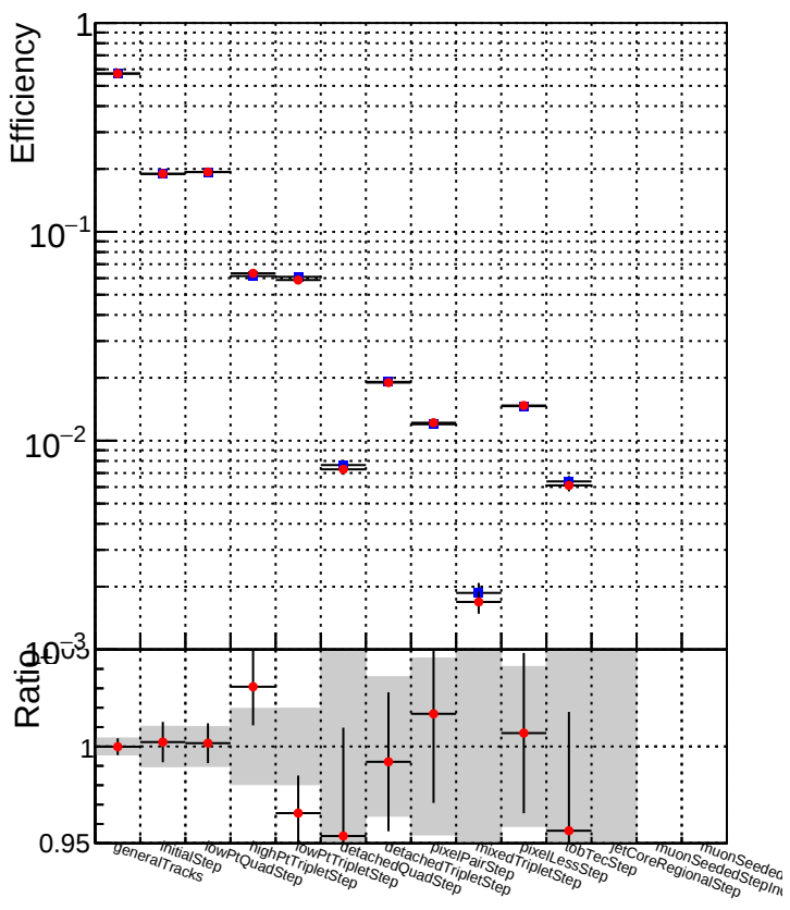
DQM_CKF_QCDHighPt_base DQM_CKF_QCDHighPt_retrainOldFiles125_v2_prelimWPM_epoch1
