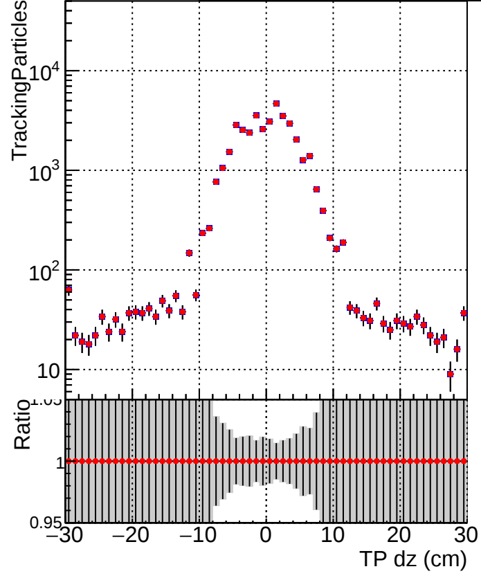
N of simulated track Legend: DQM_CKF_QCDHighPt_base (gray square) DQM_CKF_QCDHighPt_retrainOldFiles125_v2_prelimWPM_epoch1 (red circle)
