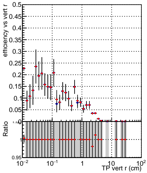
—■ DQM_CKF_QCDHighPt_base —● DQM_CKF_QCDHighPt_retrainOldFiles125_v2_prelimWPM_epoch1
