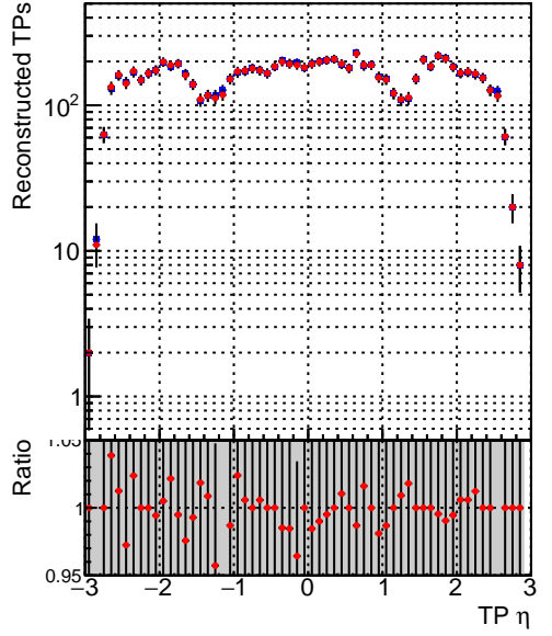
—●— DQM_CKF_QCDHighPt_base —●— DQM_CKF_QCDHighPt_retrainOldFiles125_v2_prelimWPM_epoch1
