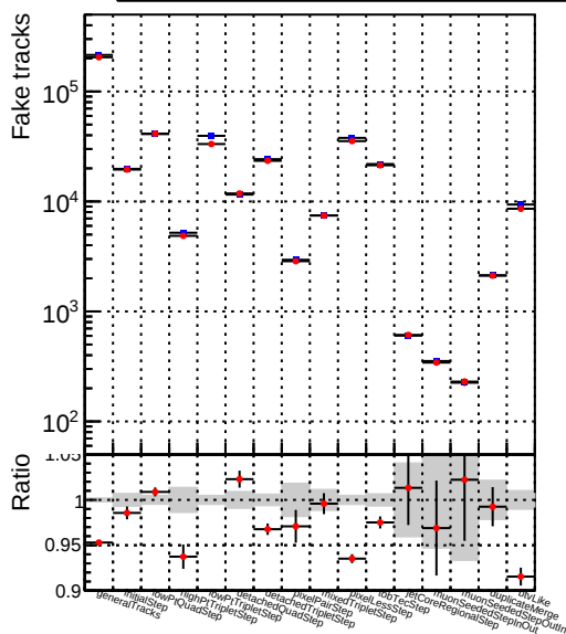
Number Model 1 DQM_CKF_QCDHighPt_retrainOldFiles125_v2_prelimWPM_epoch1
