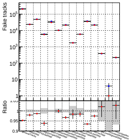
Number —●— DQM_CKF_QCDHighPt_retrainOldFiles125_v2_prelimWPM_epoch1
