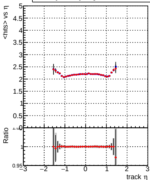
mean hits vs \eta Legend: DQM_CKF_QCDHighPt_base (blue line with error bars), DQM_CKF_QCDHighPt_retrainOldFiles125_v2_prelimWPM_epoch1 (red line with error bars)
