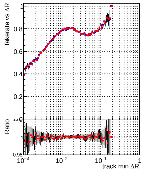
Fake rate vs \Delta R(\text{track, jet}) Legend: — DQM_CKF_QCDHighPt_base — DQM_CKF_QCDHighPt_retrainOldFiles125_v2_prelimWPM_epoch1
