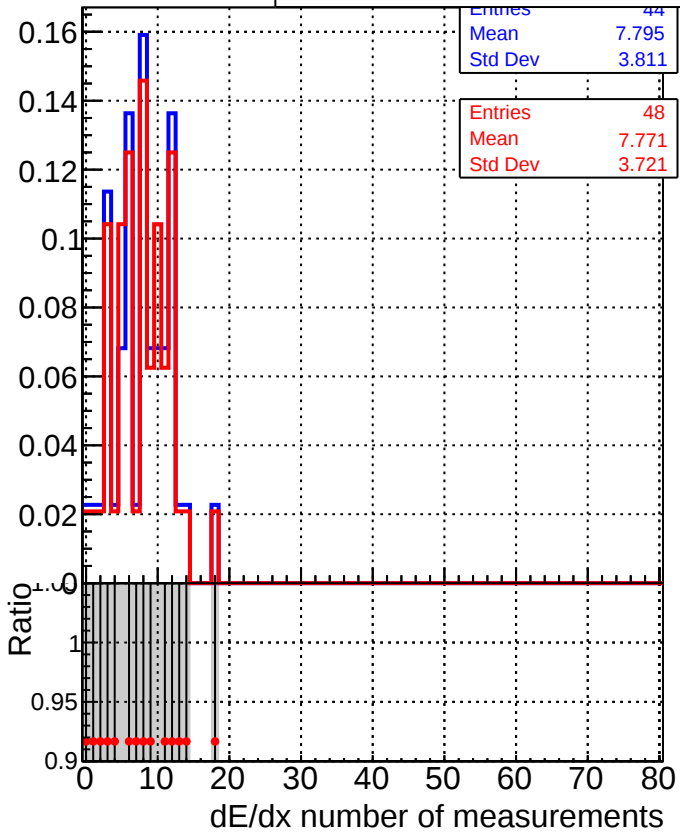
■ DQM_CKF_QCDHighPt_base ● DQM_CKF_QCDHighPt_retrainOldFiles125_v2_prelimWPM_epoch1
