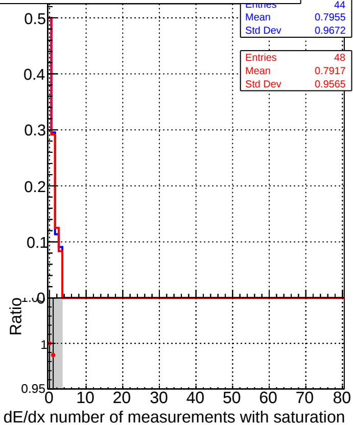
■ DQM_CKF_QCDHighPt_base ● DQM_CKF_QCDHighPt_retrainOldFiles125_v2_prelimWPM_epoch1
