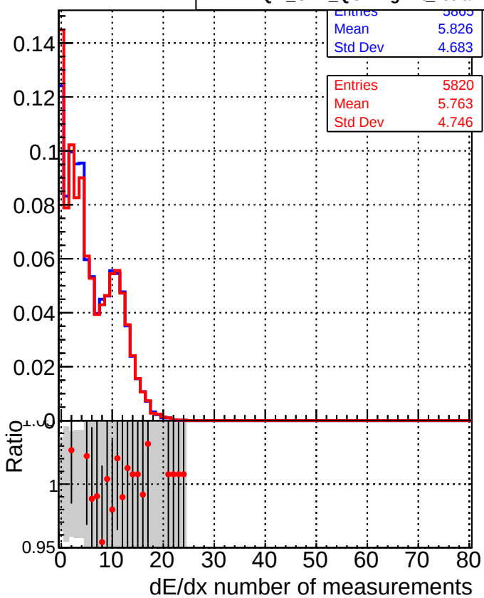
■ DQM_CKF_QCDHighPt_base ● DQM_CKF_QCDHighPt_retrainOldFiles125_v2_prelimWPM_epoch1
