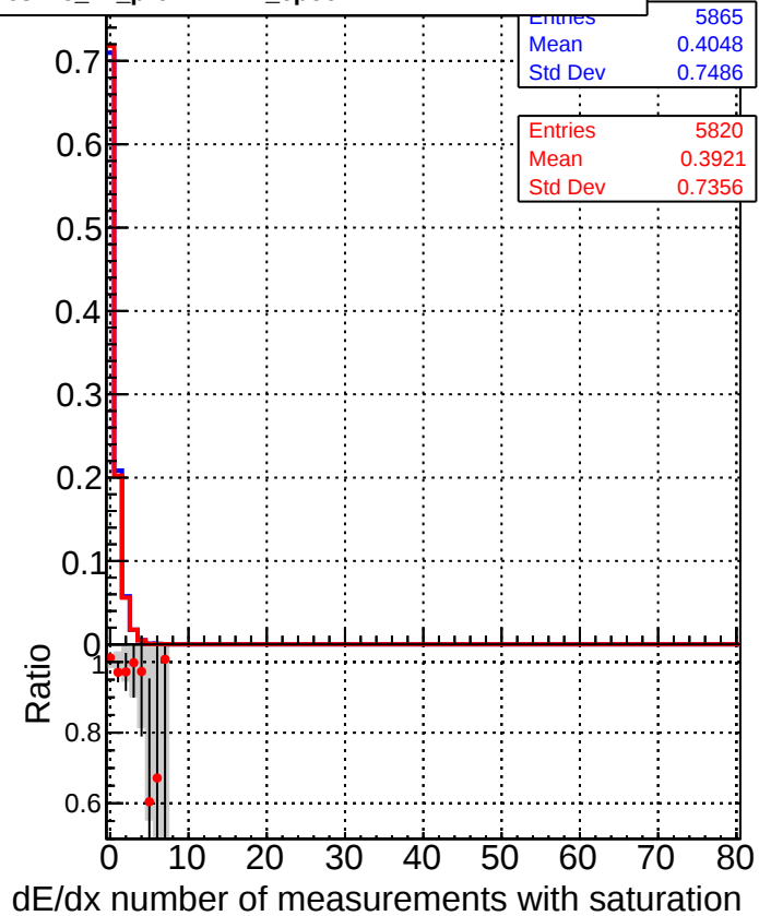
■ DQM_CKF_QCDHighPt_base ● DQM_CKF_QCDHighPt_retrainOldFiles125_v2_prelimWPM_epoch1
