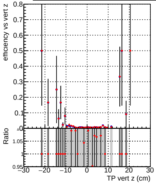
Efficiency vs vert z — DQM_CKF_QCDHighPt_base — DQM_CKF_QCDHighPt_retrainOldFiles125_v2_prelimWPM_epoch1
