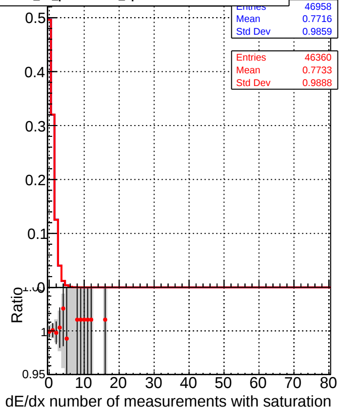
■ DQM_CKF_QCDHighPt_base ● DQM_CKF_QCDHighPt_retrainOldFiles125_v2_prelimWPM_epoch1
