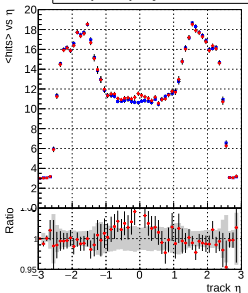
mean hits vs \eta Legend: DQM_CKF_QCDHighPt_base (blue line), DQM_CKF_QCDHighPt_retrainOldFiles125_v2_prelimWPM_epoch1 (red line)
