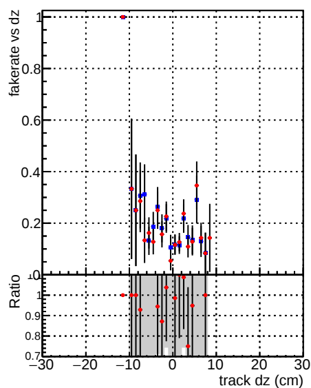
Fake rate vs dz —●— DQM_CKF_QCDHighPt_base —●— DQM_CKF_QCDHighPt_retrainOldFiles125_v2_prelimWPM_epoch1
