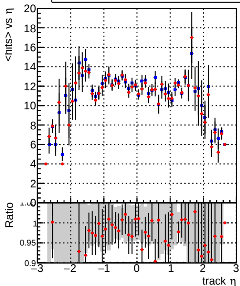
— DQM_CKF_QCDHighPt_base — DQM_CKF_QCDHighPt_retrainOldFiles125_v2_prelimWPM_epoch1 mean hits
