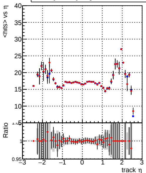
— DQM_CKF_QCDHighPt_base — DQM_CKF_QCDHighPt_retrainOldFiles125_v2_prelimWPM_epoch1 mean hits
