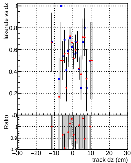
Fake rate vs dz Legend: —•— DQM CKF QCDHighPt_base —•— DQM CKF QCDHighPt_retrainOldFiles125_v2_prelimWPM_epoch1
