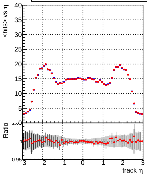
mean hits vs \eta — DQM_CKF_QCDHighPt_base — DQM_CKF_QCDHighPt_retrainOldFiles125_v2_prelimWPM_epoch1
