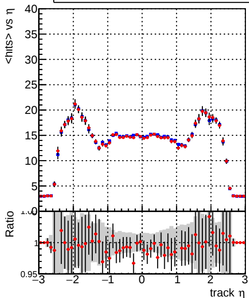
mean hits vs \eta Legend: DQM_CKF_QCDHighPt_base (blue line), DQM_CKF_QCDHighPt_retrainOldFiles125_v2_prelimWPM_epoch1 (red line)
