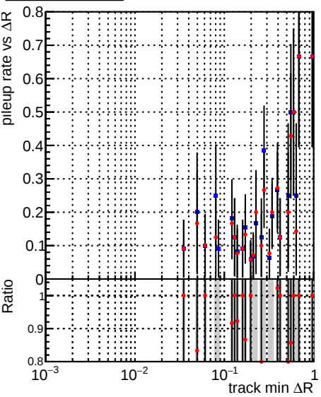
Legend: DQM_CKF_QCDHighPt_base (blue), DQM_CKF_QCDHighPt_retrainOldFiles125_v2_prelimWPM_epoch1 (red)
