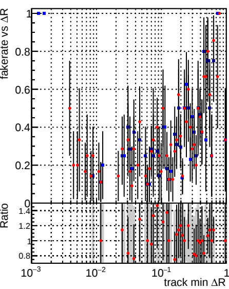
Legend: DQM_CKF_QCDHighPt_base (blue), DQM_CKF_QCDHighPt_retrainOldFiles125_v2_prelimWPM_epoch1 (red)
