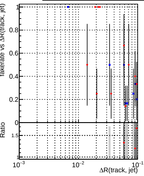
Legend: DQM_CKF_QCDHighPt_base (blue), DQM_CKF_QCDHighPt_retrainOldFiles125_v2_prelimWPM_epoch1 (red)
