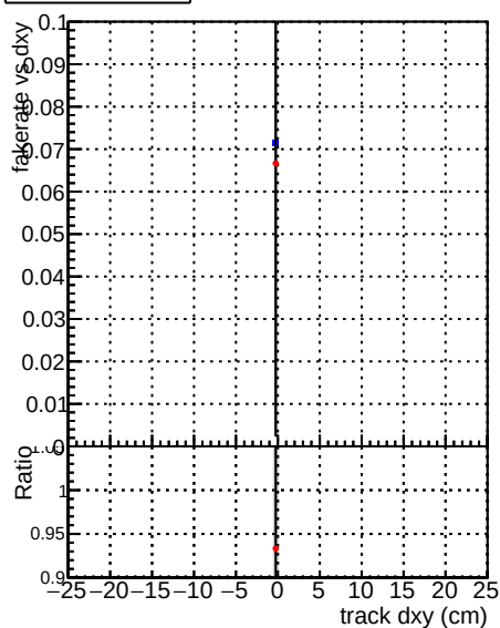
—•— DQM CKF QCDHighPt_base —•— DQM CKF QCDHighPt_retrainOldFiles125_v2_prelimWPM_epoch1
