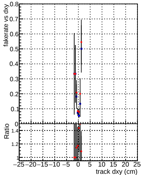
—●— DQM_CKF_QCDHighPt_base —●— DQM_CKF_QCDHighPt_retrainOldFiles125_v2_prelimWPM_epoch1
