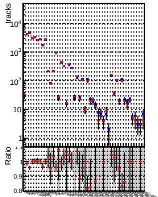
N of reco track vs. \chi^2 —●— DQM_CKF_QCDHighPt_base —●— DQM_CKF_QCDHighPt_retrainOldFiles125_v2_prelimWPM_epoch1
